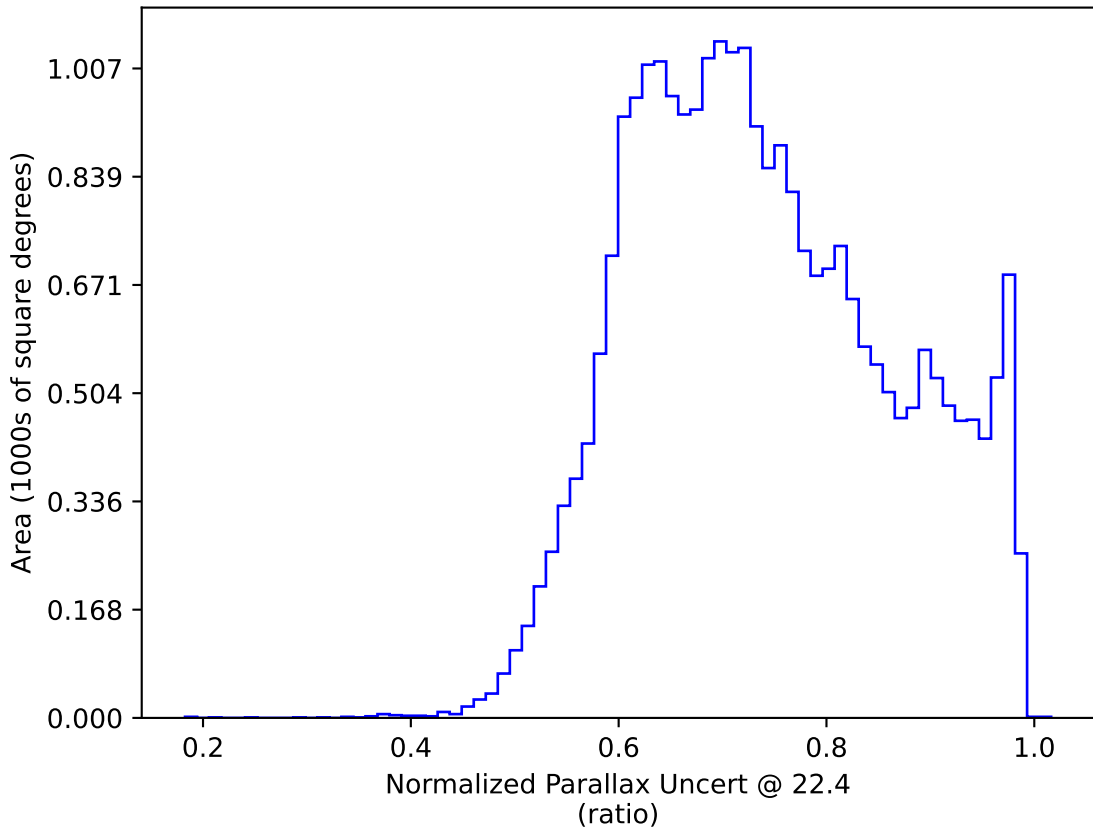
ddf_acor_sf10_lsf15_lsr10_v3.4_10yrs : Normalized Parallax Uncert @ 22.4
