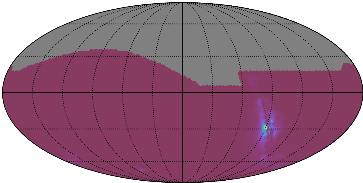
ddf_acor_sf10_lsf15_lsr10_v3.4_10yrs : NlcPoints
