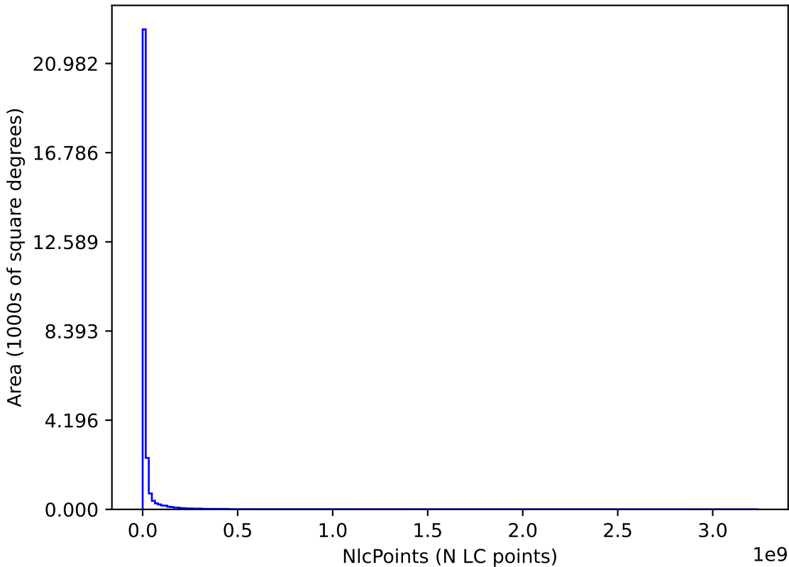
ddf_acor_sf10_lsf15_lsr10_v3.4_10yrs : NlcPoints
