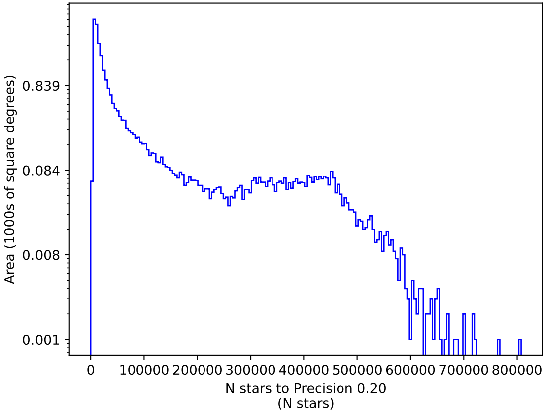
ddf_acor_sf10_lsf15_lsr10_v3.4_10yrs r: N stars to Precision 0.20
