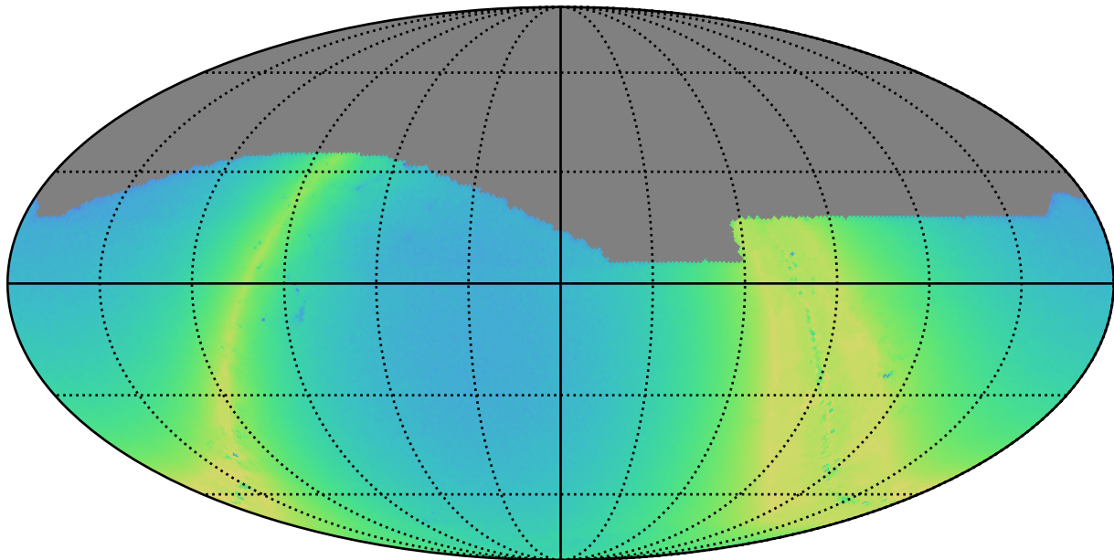
ddf_acor_sf10_lsf15_lsr10_v3.4_10yrs i: N stars to Precision 0.20
