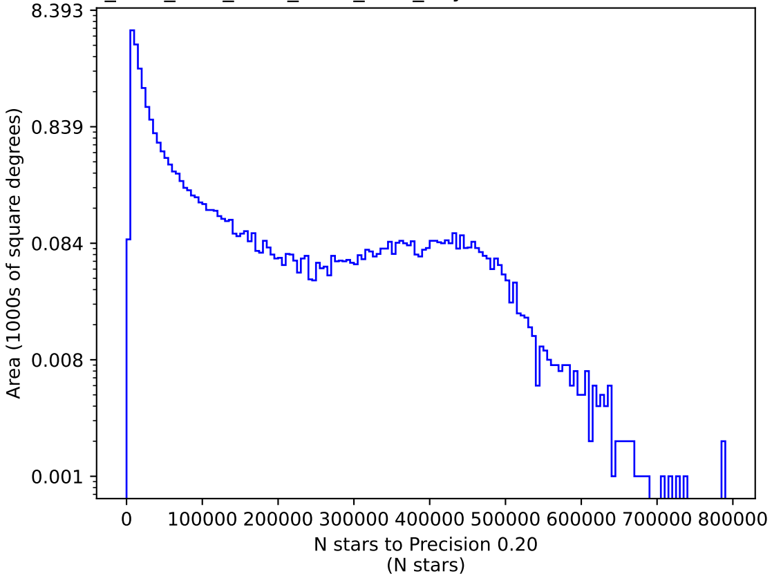
ddf_acor_sf10_lsf15_lsr10_v3.4_10yrs i: N stars to Precision 0.20
