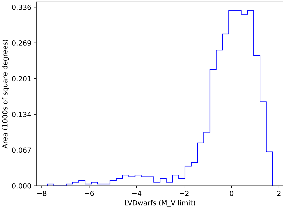
ddf_acor_sf10_lsf15_lsr10_v3.4_10yrs gi SCP: LVDwarfs
