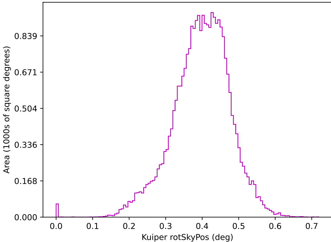
ddf_acor_sf10_lsf15_lsr10_v3.4_10yrs z: Kuiper rotSkyPos
