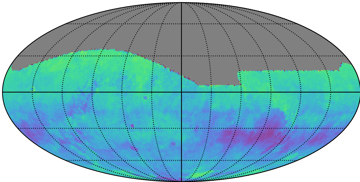
ddf_acor_sf10_lsf15_lsr10_v3.4_10yrs r: Kuiper rotSkyPos
