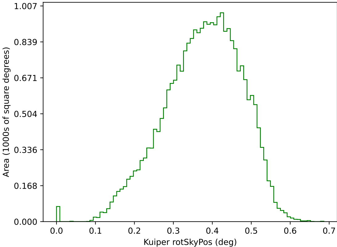
ddf_acor_sf10_lsf15_lsr10_v3.4_10yrs g: Kuiper rotSkyPos
