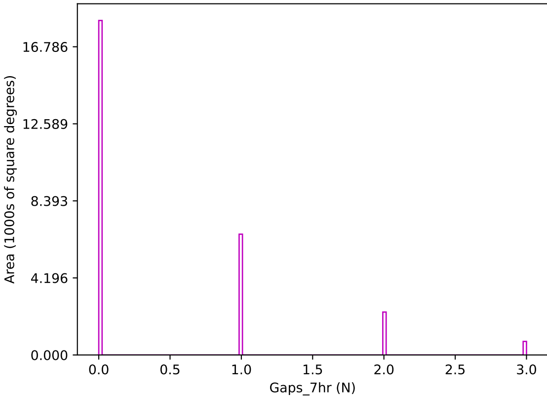
ddf_acor_sf10_ls15_lsr10_v3.4_10yrs z band: Gaps_7hr
