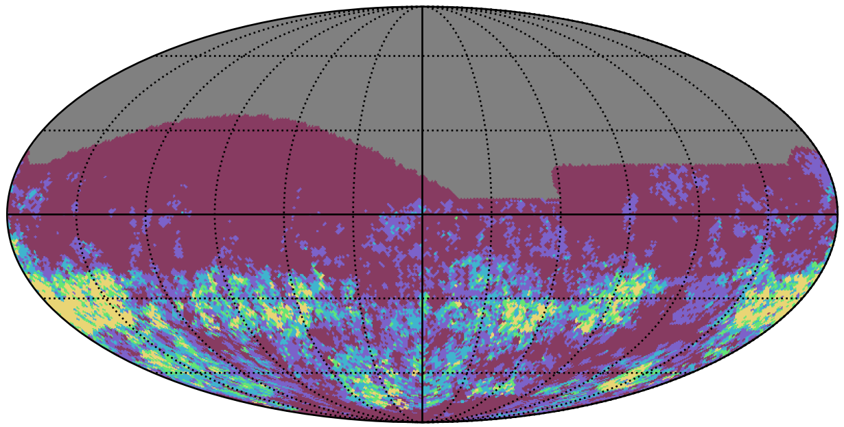
ddf_acor_sf10_lsf15_lsr10_v3.4_10yrs r band: Gaps_7hr
