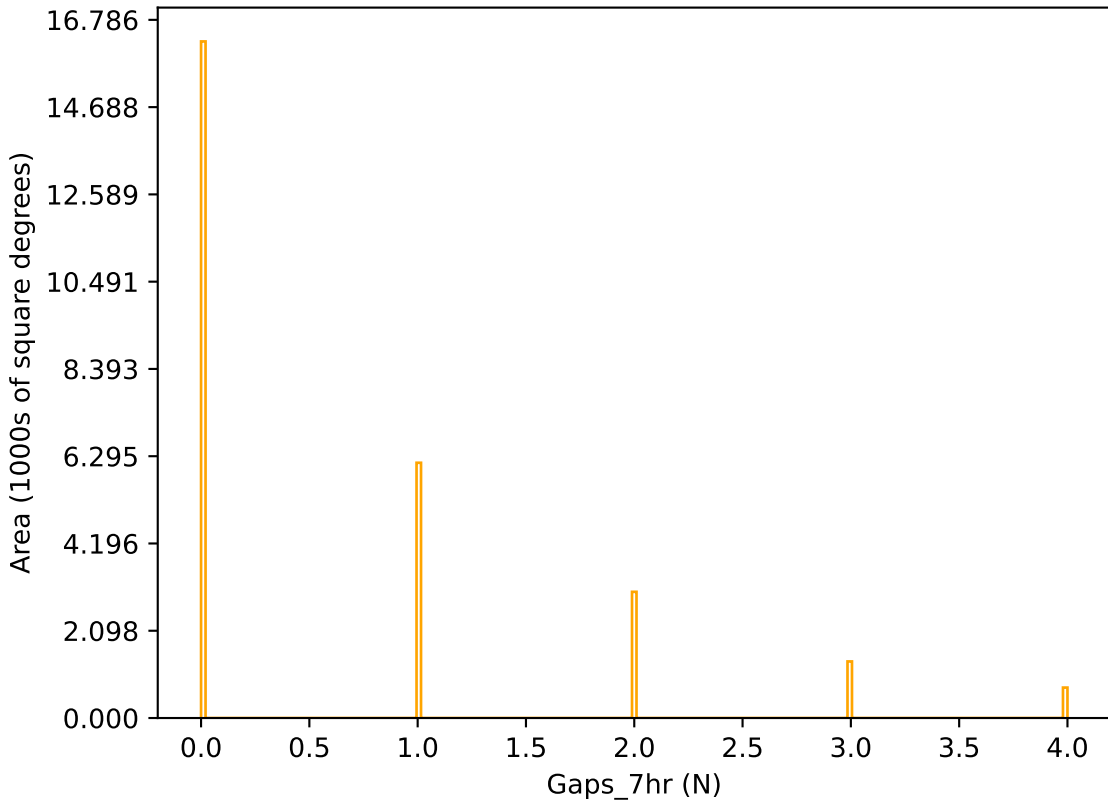
ddf_acor_sf10_lsf15_lsr10_v3.4_10yrs r band: Gaps_7hr
