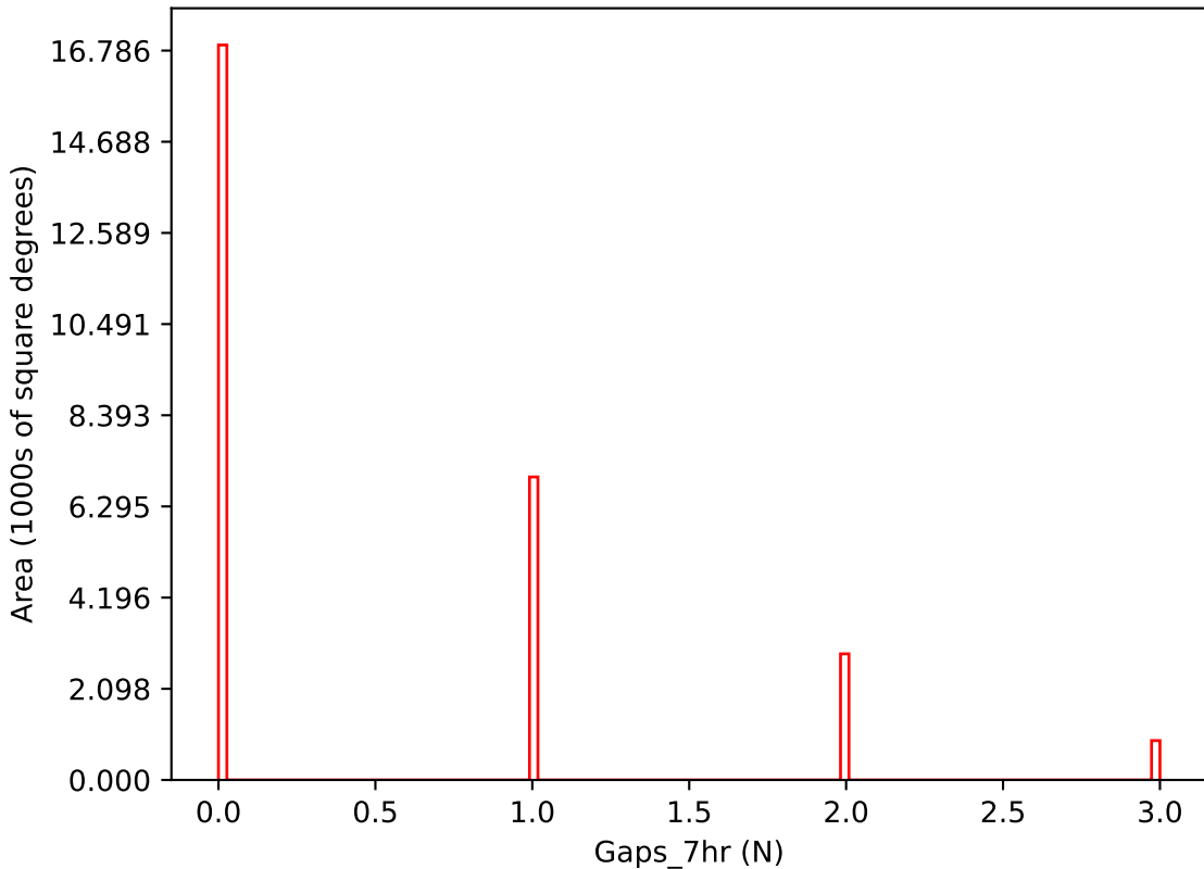
ddf_acor_sf10_lsf15_lsr10_v3.4_10yrs i band: Gaps_7hr
