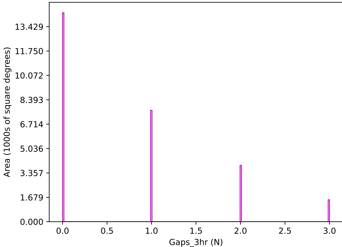
ddf_acor_sf10_ls15_lsr10_v3.4_10yrs z band: Gaps_3hr
