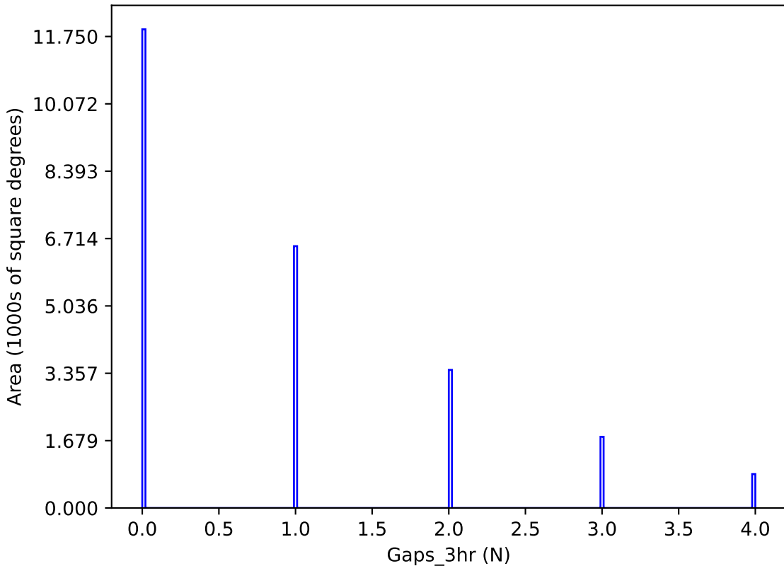
ddf_acor_sf10_ls15_lsr10_v3.4_10yrs y band: Gaps_3hr
