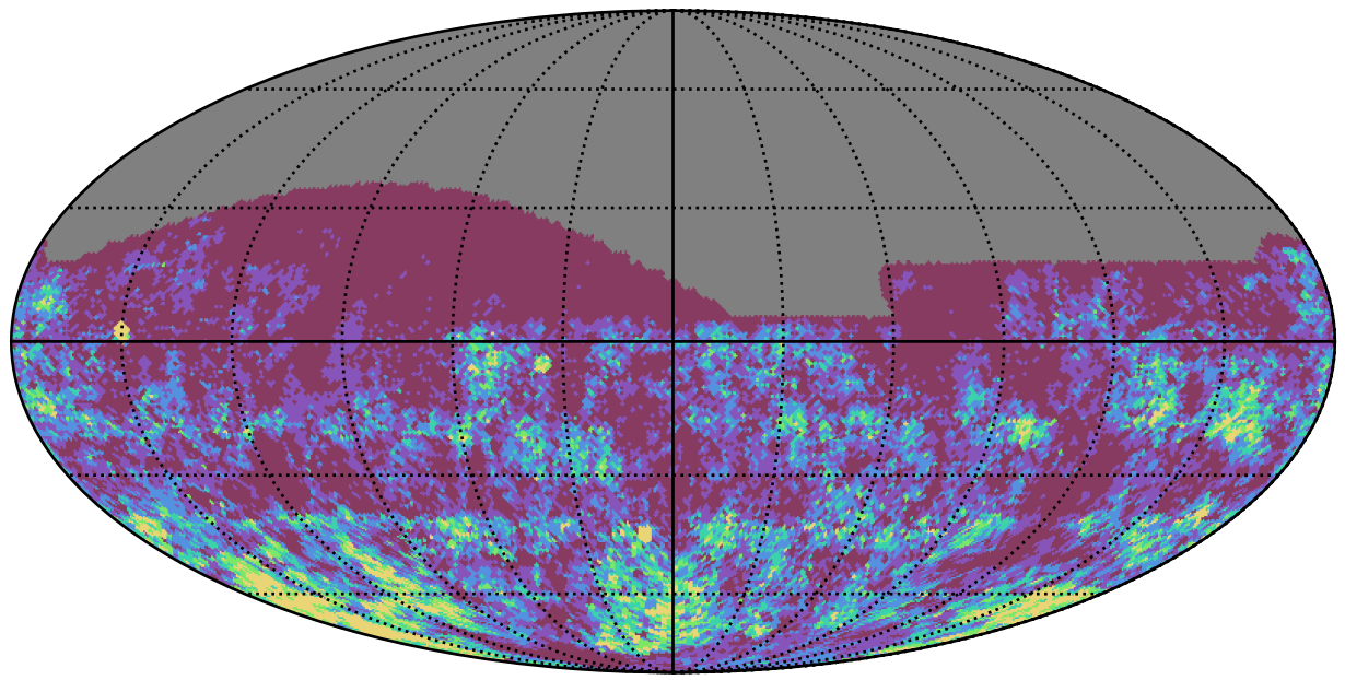
ddf_acor_sf10_ls15_lsr10_v3.4_10yrs r band: Gaps_3hr
