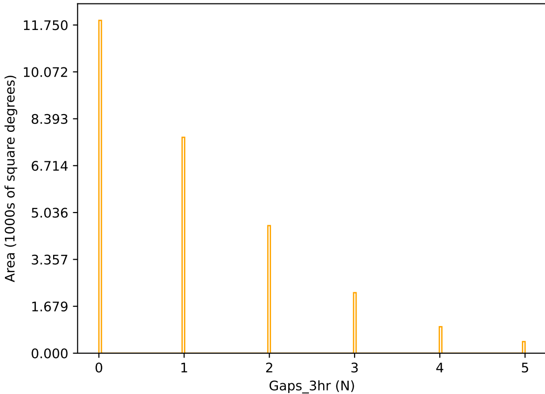
ddf_acor_sf10_lsf15_lsr10_v3.4_10yrs r band: Gaps_3hr
