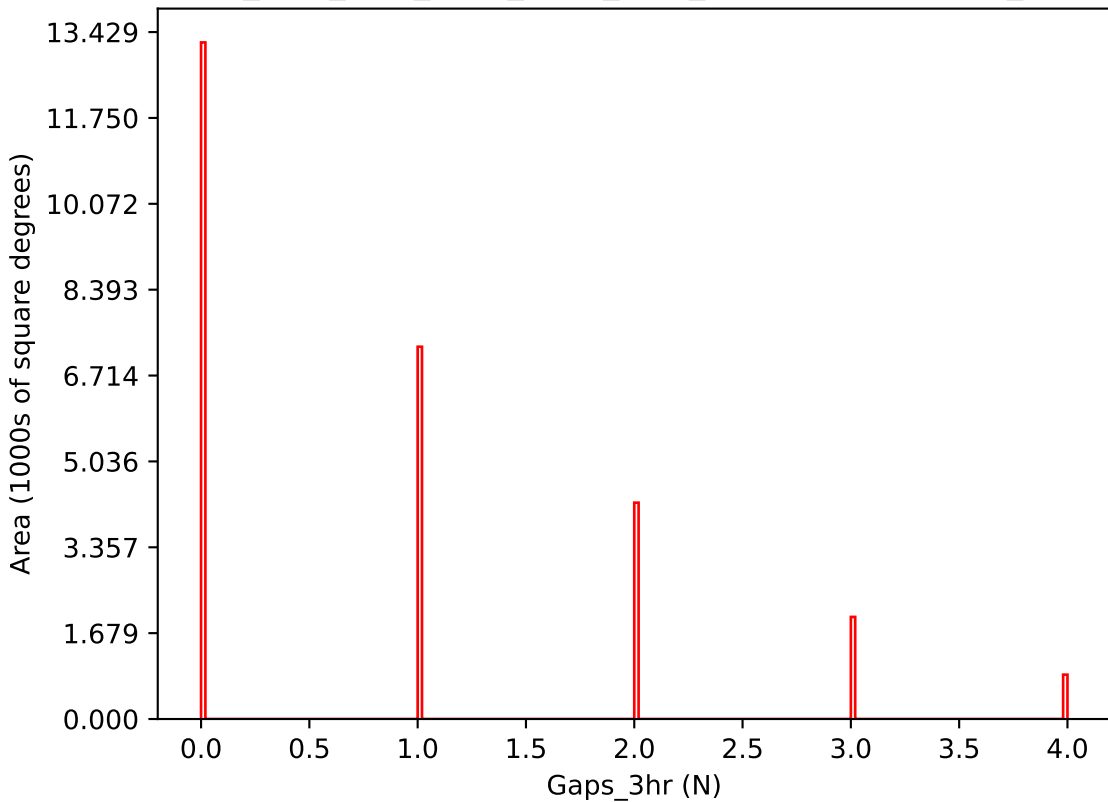
ddf_acor_sf10_lsf15_lsr10_v3.4_10yrs i band: Gaps_3hr
