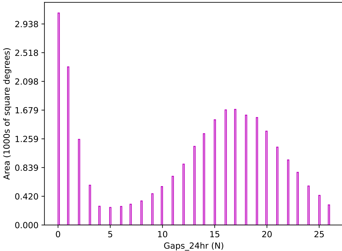
ddf_acor_sf10_ls15_lsr10_v3.4_10yrs z band: Gaps_24hr
