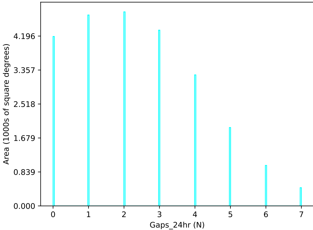
ddf_acor_sf10_lsf15_lsr10_v3.4_10yrs u band: Gaps_24hr
