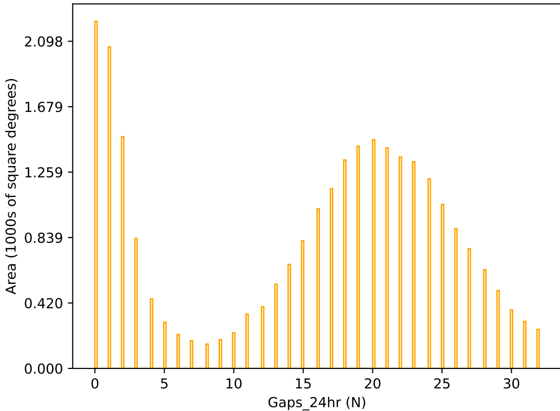
ddf_acor_sf10_ls15_lsr10_v3.4_10yrs r band: Gaps_24hr
