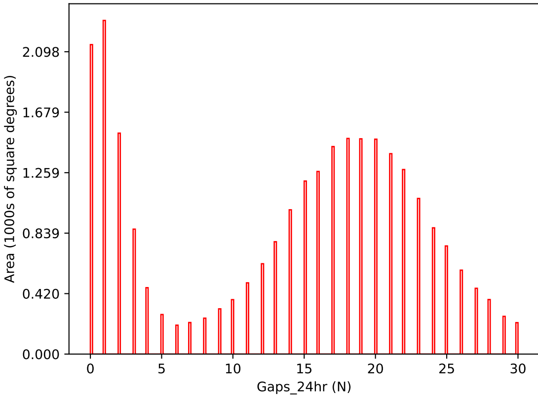
ddf_acor_sf10_ls15_lsr10_v3.4_10yrs i band: Gaps_24hr
