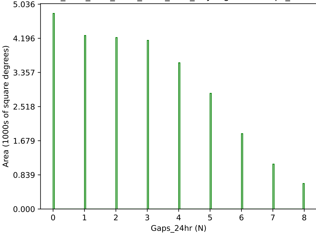
ddf_acor_sf10_lsf15_lsr10_v3.4_10yrs g band: Gaps_24hr
