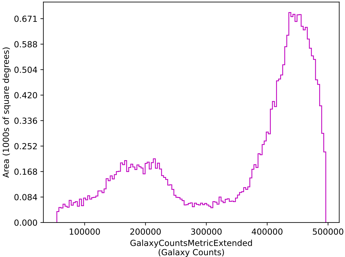
ddf_acor_sf10_lsf15_lsr10_v3.4_10yrs z: GalaxyCountsMetricExtended
