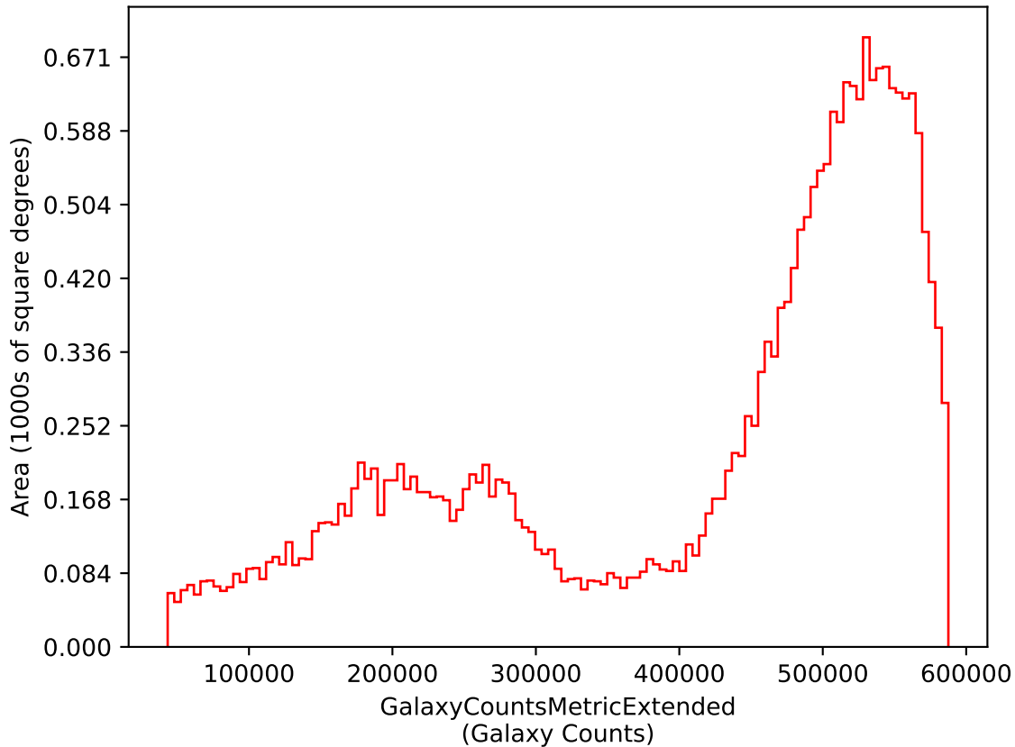
ddf_acor_sf10_lsf15_lsr10_v3.4_10yrs i: GalaxyCountsMetricExtended
