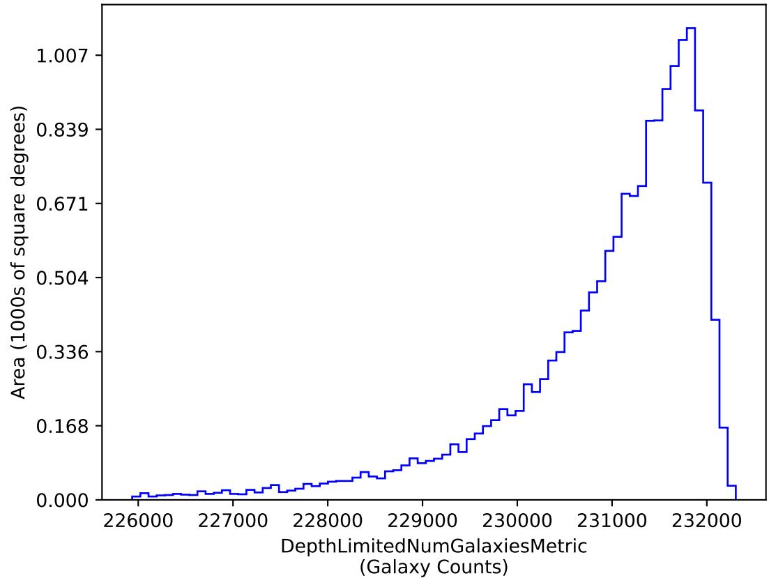
ddf_acor_sf10_ls15_lsr10_v3.4_10yrs i band galaxies non-DD: DepthLimitedNumGalaxiesMetric
