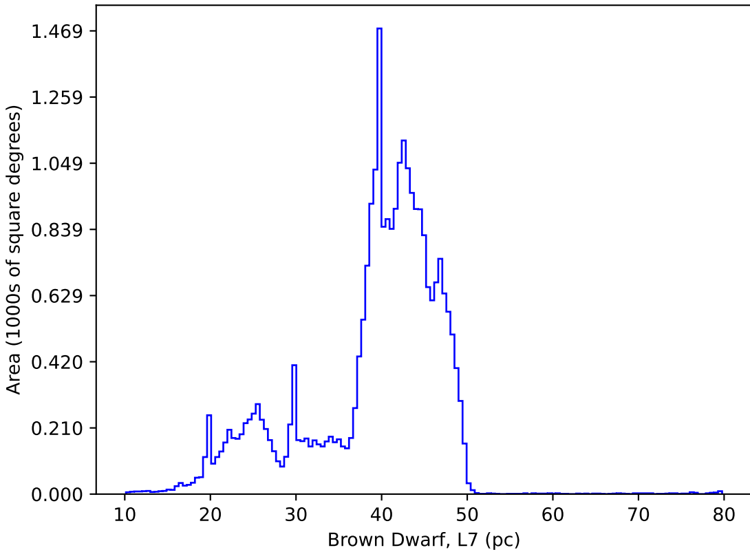
ddf_acor_sf10_lsf15_lsr10_v3.4_10yrs : Brown Dwarf, L7
