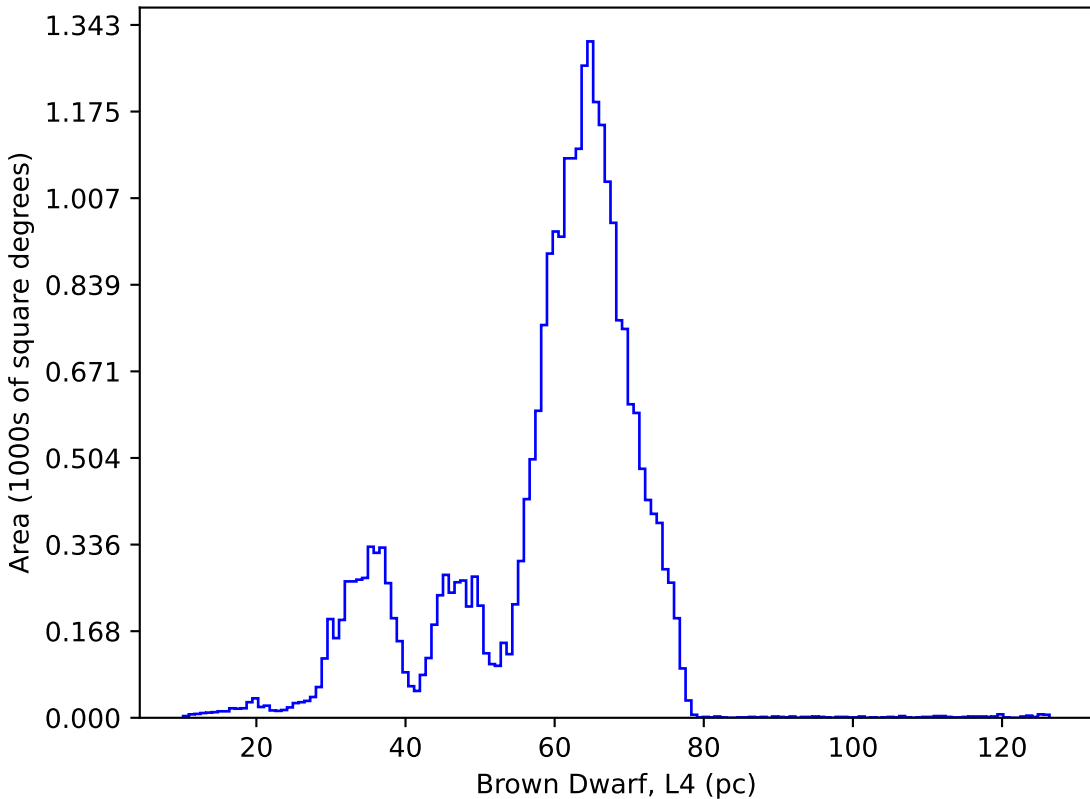
ddf_acor_sf10_lsf15_lsr10_v3.4_10yrs : Brown Dwarf, L4
