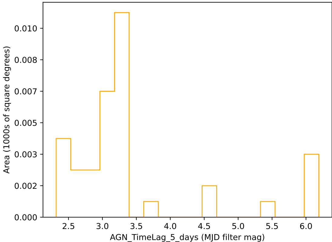
ddf_acor_sf10_lsf15_lsr10_v3.4_10yrs r band: AGN_TimeLag_5_days
