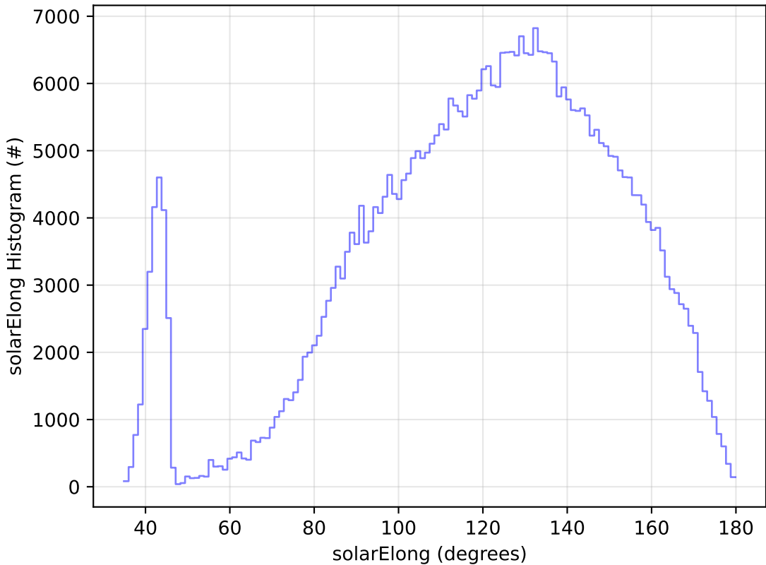
ddf_acor_sf10_ls15_lsr10_v3.4_10yrs WFD z band: solarElong Histogram
