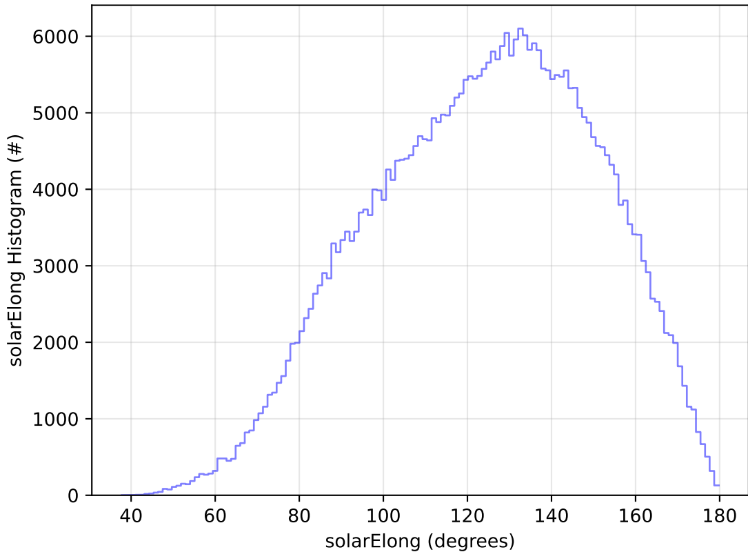
ddf_acor_sf10_lsf15_lsr10_v3.4_10yrs WFD y band: solarElong Histogram
