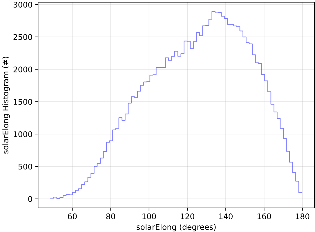
ddf_acor_sf10_lsf15_lsr10_v3.4_10yrs WFD u band: solarElong Histogram
