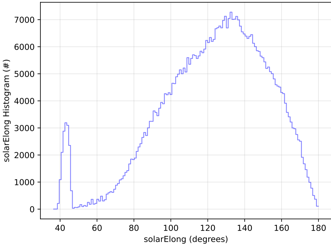
ddf_acor_sf10_ls15_lsr10_v3.4_10yrs WFD r band: solarElong Histogram
