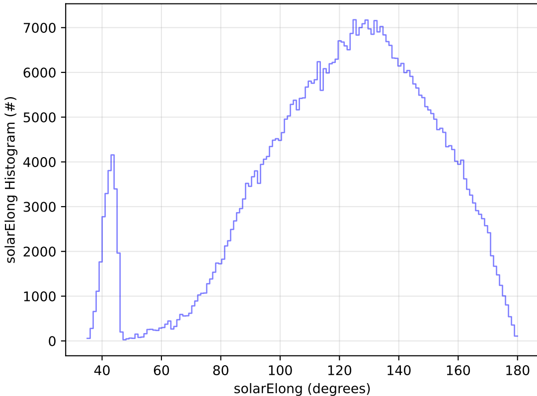
ddf_acor_sf10_lsf15_lsr10_v3.4_10yrs WFD i band: solarElong Histogram
