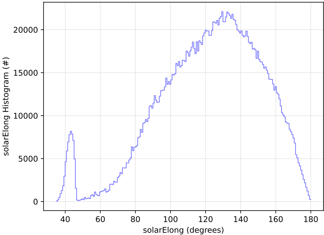
ddf_acor_sf10_lsf15_lsr10_v3.4_10yrs WFD all bands: solarElong Histogram
