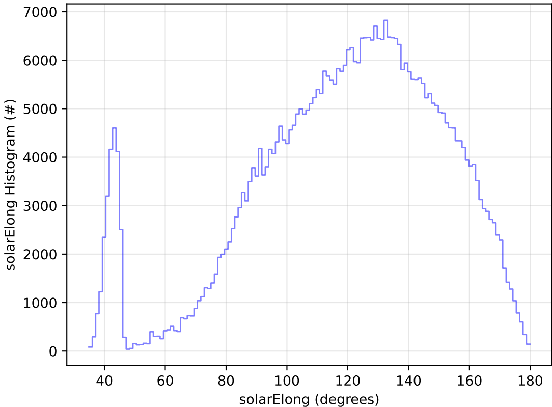
ddf_acor_sf10_lsf15_lsr10_v3.4_10yrs All sky z band: solarElong Histogram
