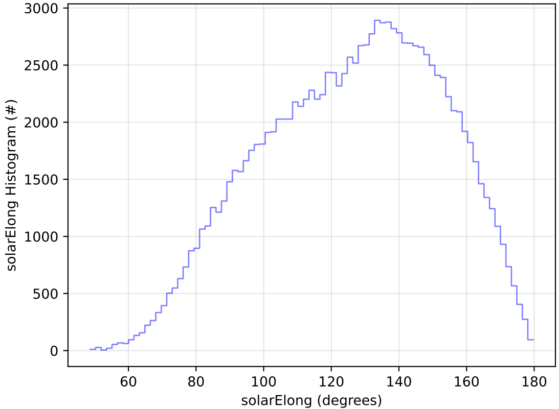
ddf_acor_sf10_lsf15_lsr10_v3.4_10yrs All sky u band: solarElong Histogram
