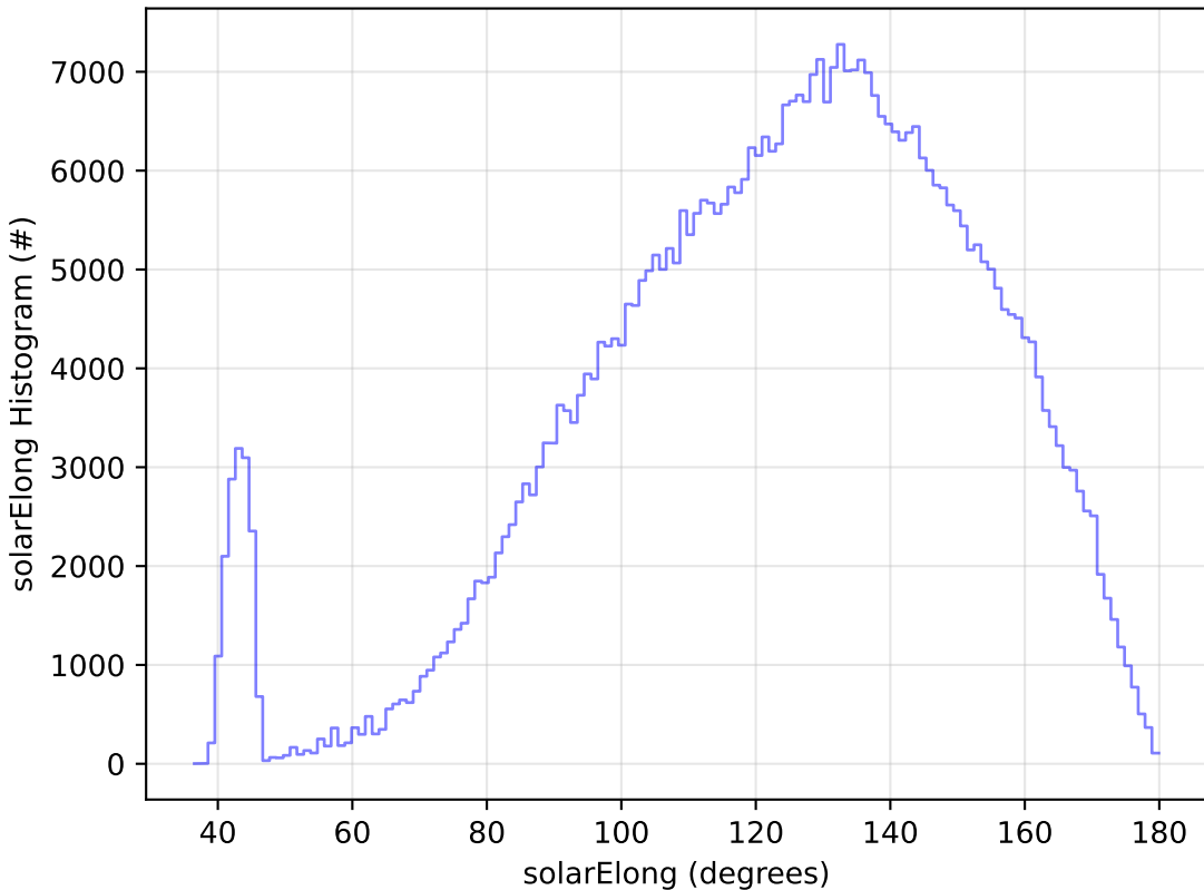
ddf_acor_sf10_lsf15_lsr10_v3.4_10yrs All sky r band: solarElong Histogram
