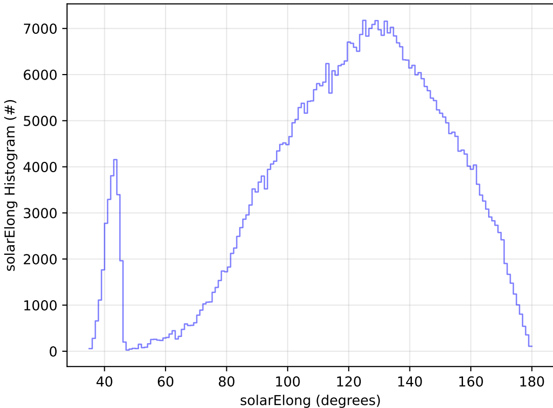
ddf_acor_sf10_lsf15_lsr10_v3.4_10yrs All sky i band: solarElong Histogram
