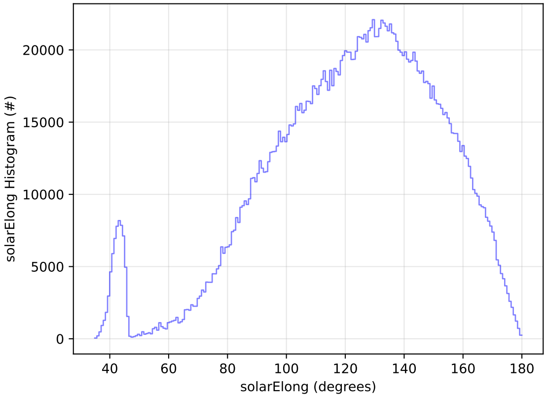
ddf_acor_sf10_lsf15_lsr10_v3.4_10yrs All sky all bands: solarElong Histogram
