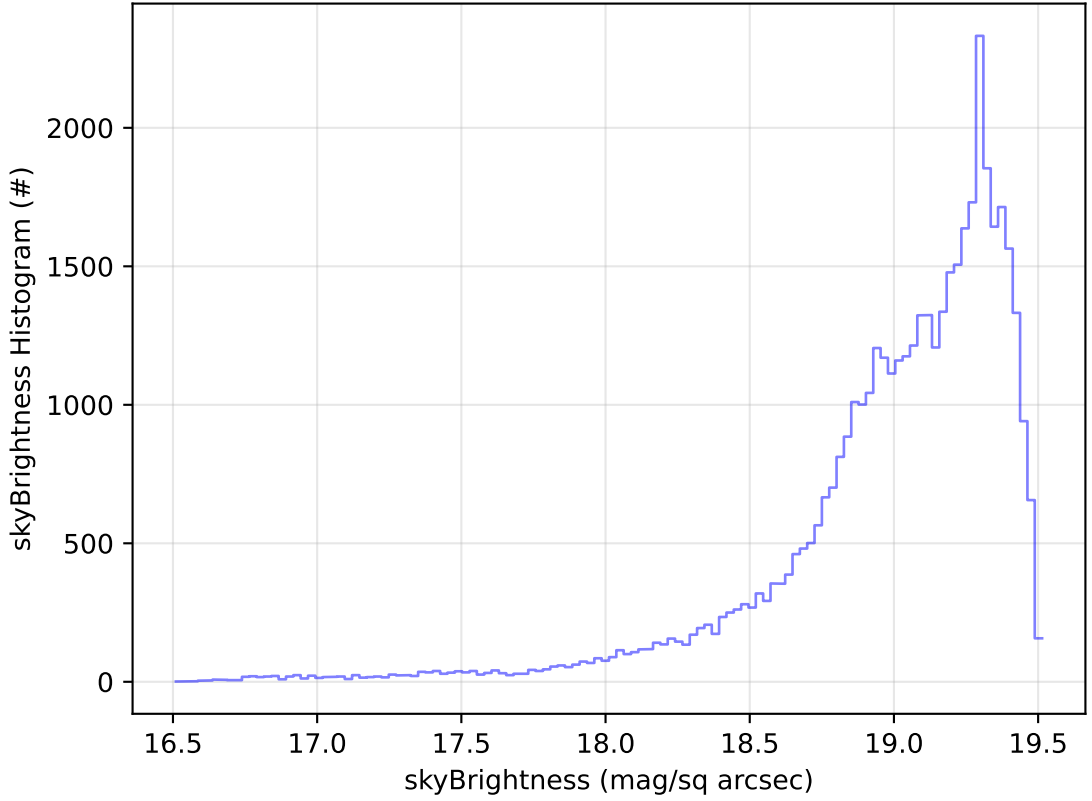
ddf_acor_sf10_lsf15_lsr10_v3.4_10yrs Yr 1 z band: skyBrightness Histogram
