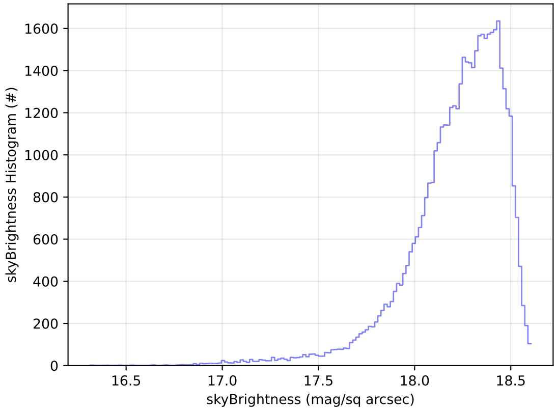
ddf_acor_sf10_lsf15_lsr10_v3.4_10yrs Yr 1 y band: skyBrightness Histogram
