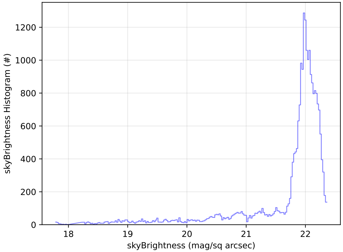
ddf_acor_sf10_lsf15_lsr10_v3.4_10yrs Yr 1 g band: skyBrightness Histogram
