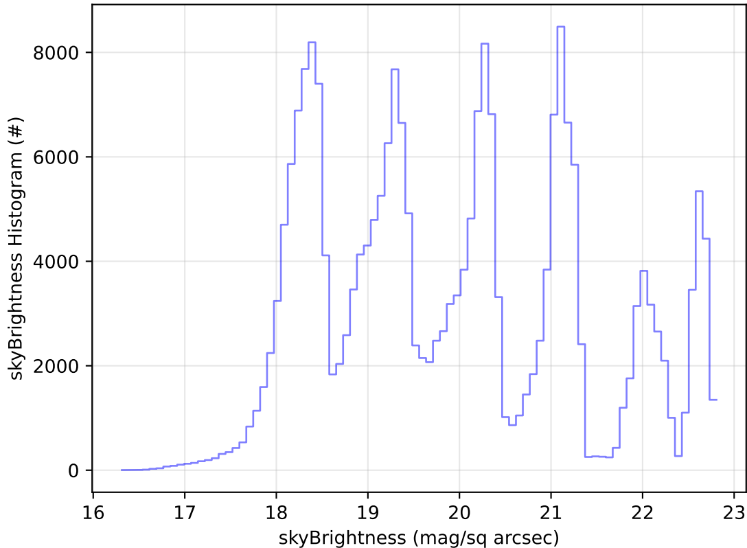
ddf_acor_sf10_lsf15_lsr10_v3.4_10yrs Yr 1 all bands: skyBrightness Histogram
