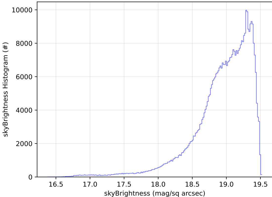
ddf_acor_sf10_lsf15_lsr10_v3.4_10yrs WFD z band: skyBrightness Histogram
