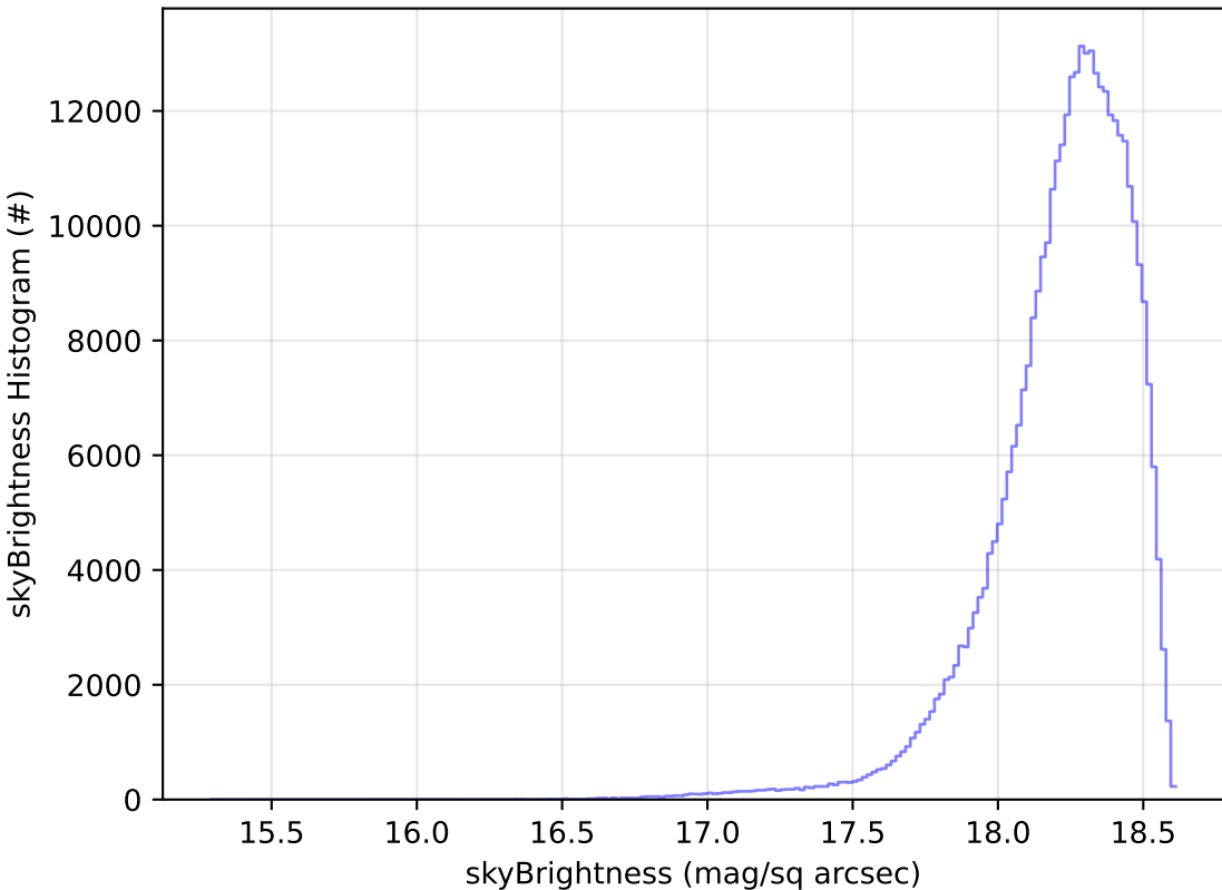
ddf_acor_sf10_lsf15_lsr10_v3.4_10yrs WFD y band: skyBrightness Histogram
