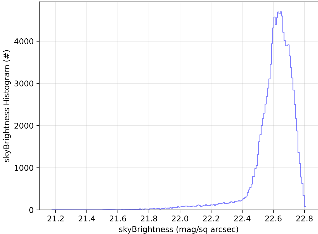
ddf_acor_sf10_lsf15_lsr10_v3.4_10yrs WFD u band: skyBrightness Histogram
