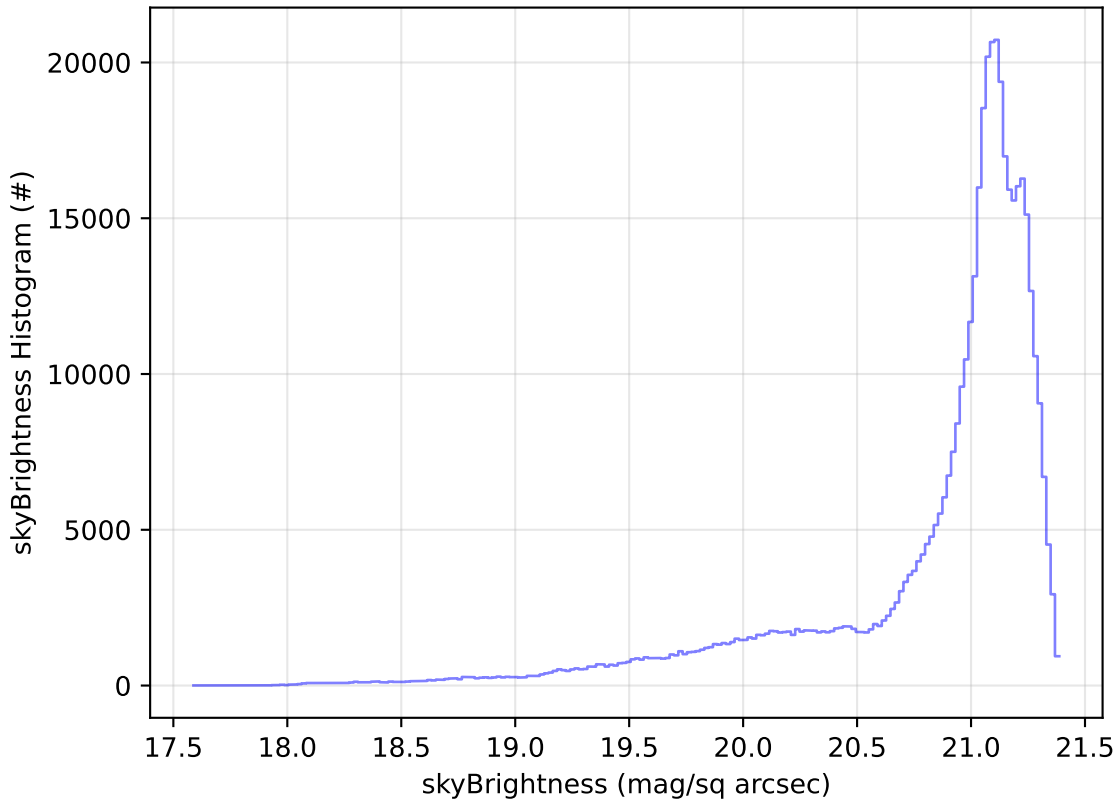
ddf_acor_sf10_lsf15_lsr10_v3.4_10yrs WFD r band: skyBrightness Histogram
