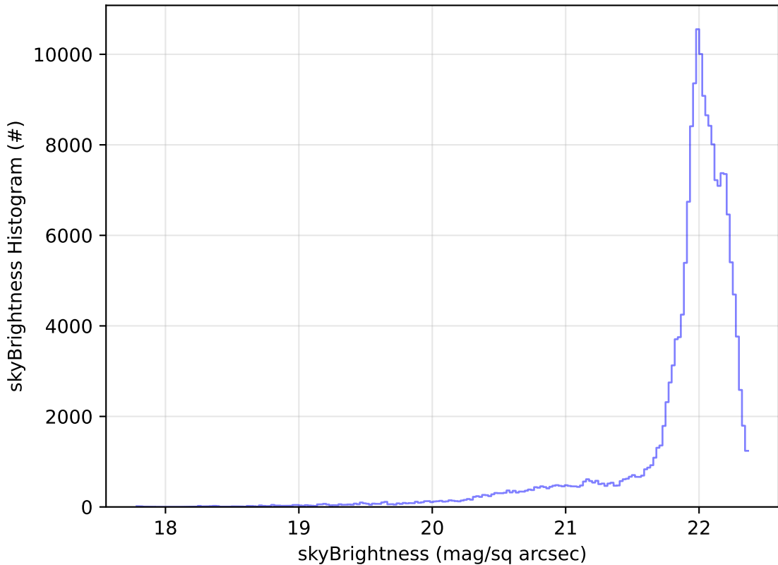
ddf_acor_sf10_lsf15_lsr10_v3.4_10yrs WFD g band: skyBrightness Histogram
